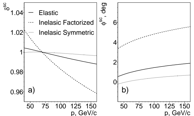
FIG. 28: Kaon momentum dependence of screening corrections to (a:) the magnitude and (b:) the phase of f_-(p) , for various models from [38]. The magnitude of each correction is defined to be 1 at 70 GeV/c.
