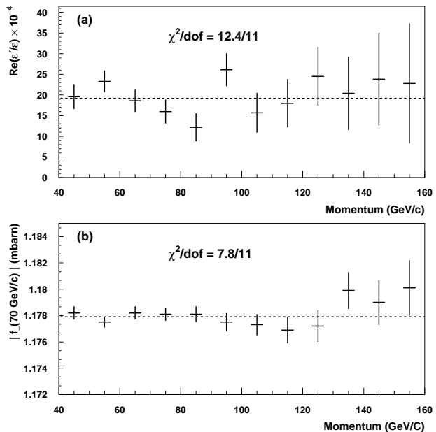
FIG. 23: (a) Re(\epsilon'/\epsilon) and (b) |f_-(70 \text{ GeV}/c)| in 10 GeV/c momentum bins. All points are statistically independent. The dashed lines indicate the values for the full data sample.
