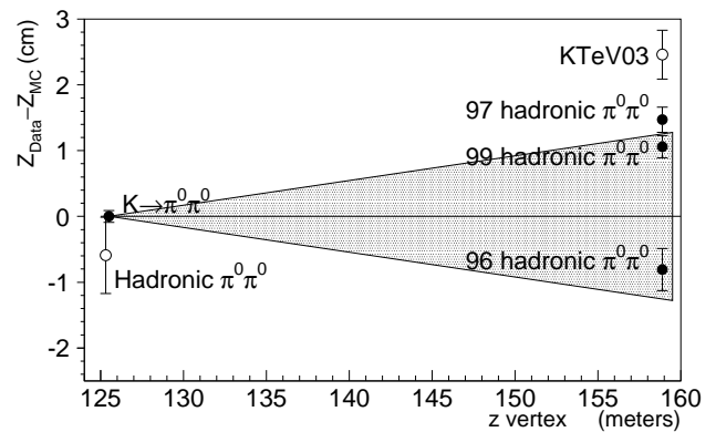
FIG. 15: Energy scale tests at the regenerator and vacuum window. The difference between the reconstructed z positions for data and MC is plotted for K \rightarrow \pi^0\pi^0 events, and for hadronically produced \pi^0\pi^0 pairs at the regenerator and the downstream detector elements. The solid point at the regenerator edge is the K \rightarrow \pi^0\pi^0 sample; there is no difference between data and MC by construction. The open point at the regenerator edge is the average shift of the hadronic regenerator samples for all three datasets. The points at the vacuum window are the shifts for the downstream hadronic events for each dataset separately. The shaded region shows the range of data-MC shifts covered by the total systematic uncertainty from the energy scale. For reference, the data-MC shift at the vacuum window from KTeV03 is also plotted.
