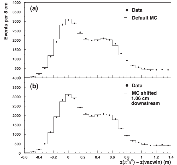
FIG. 16: z -vertex distributions of \pi^0\pi^0 pairs produced hadronically in downstream detector elements for 1999 data and MC. (a) Data (dots) and nominal MC (histogram). (b) Data (dots) and MC that is shifted 1.06 cm downstream to match the data (histogram).
