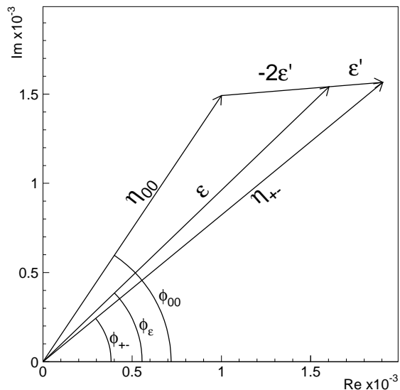
FIG. 1: Diagram of CP violating kaon parameters. For this illustration, the \epsilon parameter has the central value measured by KTeV and the value of \epsilon' is scaled by a factor of 50. Although they appear distinct in this diagram, note that \phi_{+-} and \phi_{00} are consistent with each other within experimental errors.
