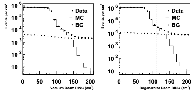
FIG. 11: K \rightarrow \pi^0\pi^0 RING distributions for data and signal MC in the vacuum (left) and regenerator (right) beams. The dashed line indicates our cut.
