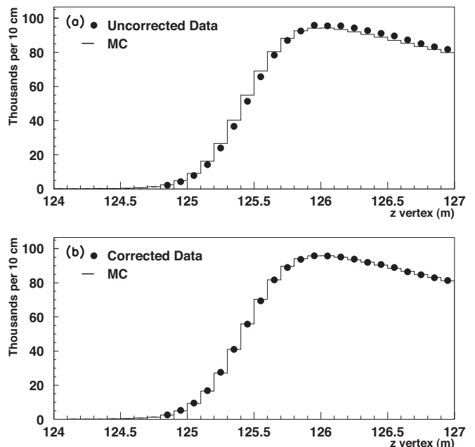
FIG. 13: Regenerator beam K \rightarrow \pi^0 \pi^0 z vertex distribution near the regenerator for 1999 data and Monte Carlo. (a) Uncorrected data. (b) Data with energy scale correction applied.
