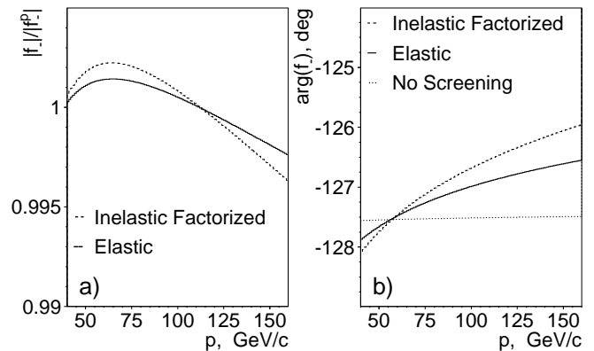
FIG. 29: Kaon momentum dependence of (a:) ratio of |f_-(p)| from the fits using elastic (solid line) and inelastic factorized (dashed line) screening corrections to |f_-^P(p)| from the fit using no screening corrections; (b:) \arg(f_-(p)) from the fits with elastic (solid line), inelastic (dashed line) screening corrections and with no screening corrections (dotted line).
